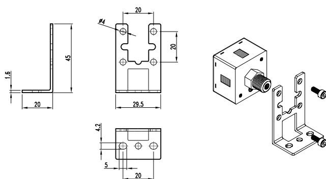
MOUNTING BRACKET L TYPE SUPPORT DE MONTAGE TYPE L STAFFA DI MONTAGGIO A L
